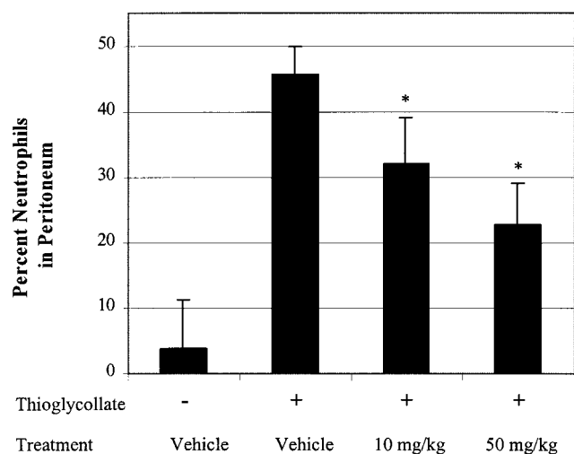
Figure 6. Treatment with compound 29 at 10 and 50 mg/kg reduces neutrophil influx in an in vivo model of inflammation. Balb/c mice were dosed with compound or vehicle (buffered saline) by intravenous injection immediately before intraperitoneal challenge with thioglycollate. Total cells and neutrophils in the peritoneum were quantified 4 h later ( n = 4-5 mice per group). * p < 0.01 by unpaired, two-tailed t -test.
