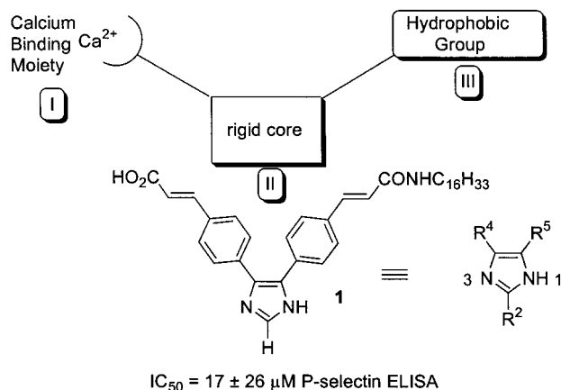
Figure 2. Criteria believed to be essential for a potent selectin inhibitor.
