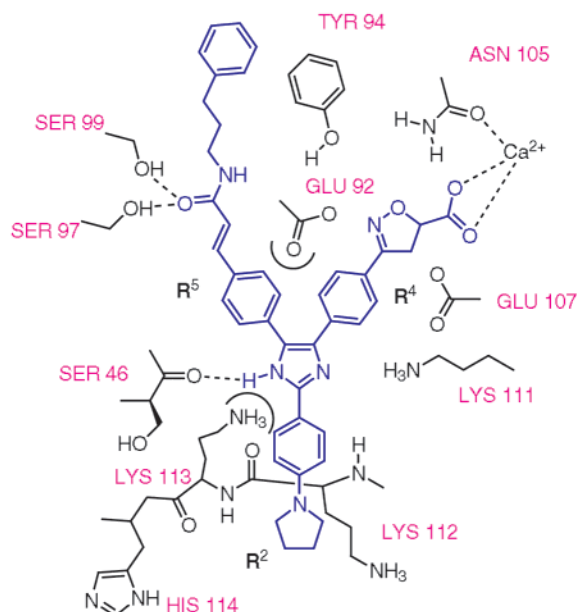
Figure 4. Schematic representation of 14 showing the proposed interactions with the P-selectin binding site.
