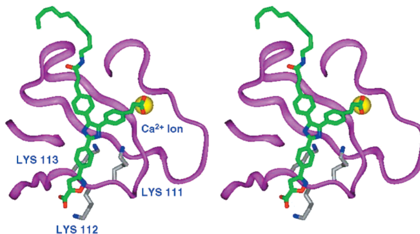
Figure 5. Stereoview of compound 29 bound to P-selectin illustrating the proposed binding mode.
