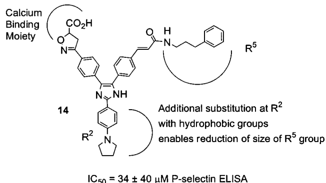
Figure 3. Additional substitution at R 2 allows reduction in size of the R 5 substituent.
